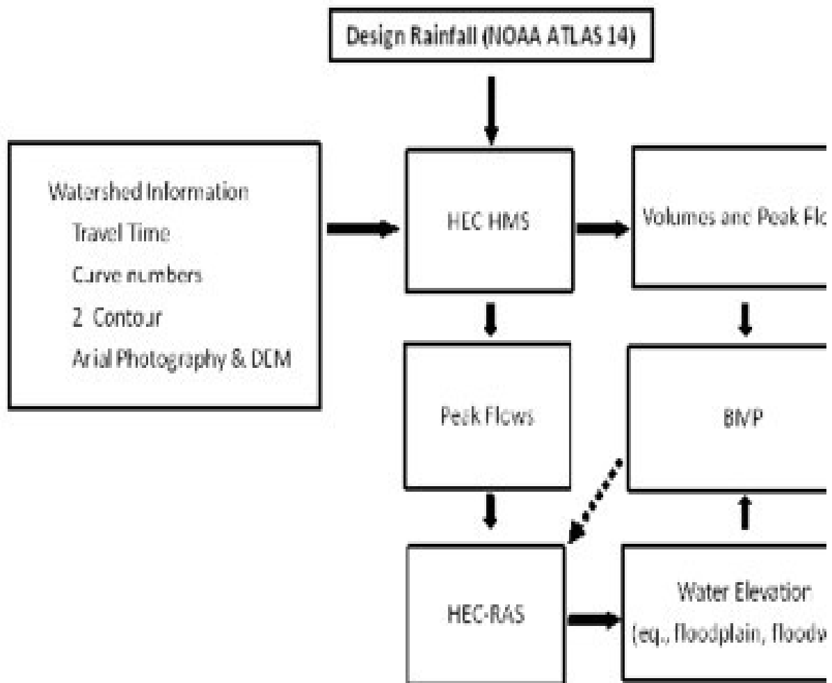
Figure 3 - Hydrologic Modeling Flow Diagram
