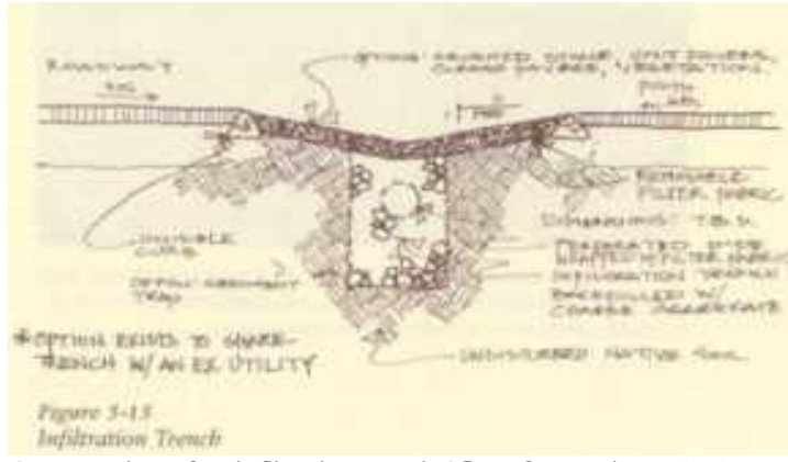
Cross-section of an infiltration trench ( Green Streets , Figure 5-15, page 59)
